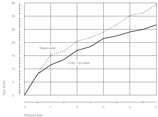
Nobili Widd® 35 Eco flow graph compiled by the Nobili laboratory on 15/10/2009. Test conditions: cold water at 15°C, hot water at 65°C.
