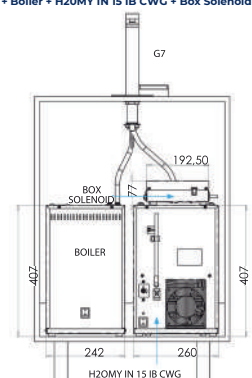
Pro-Stream hot, Cold & Sparkling G7 + Boiler + H20MY IN 15 IB CWG + Box Solenoid CWG
