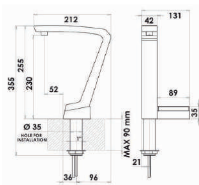
Size of G7 Faucet
